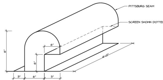
ELEVATION (FOR THE INTENT)
